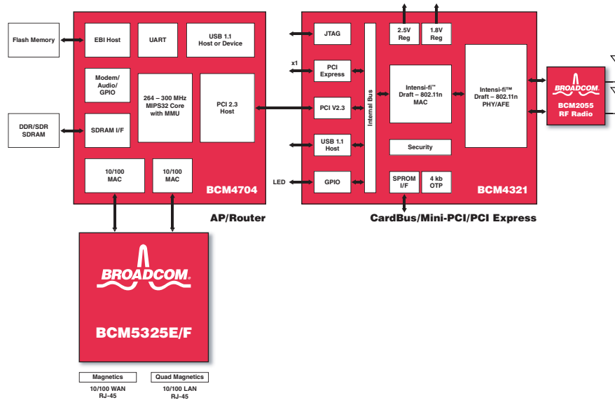
BCM4321 and BCM2055 AP/Router Block Diagram
